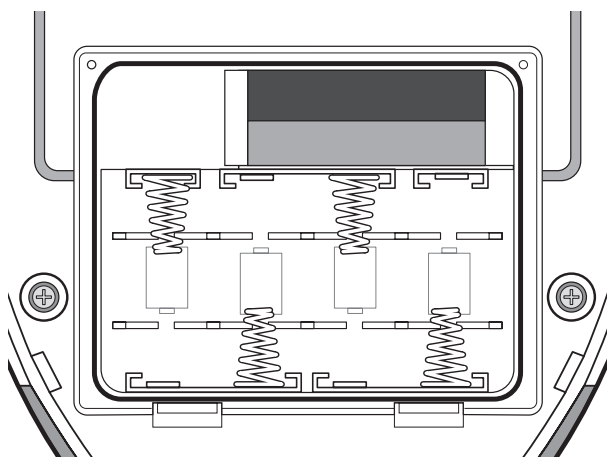
Rear view of Dummy Siren Unit
