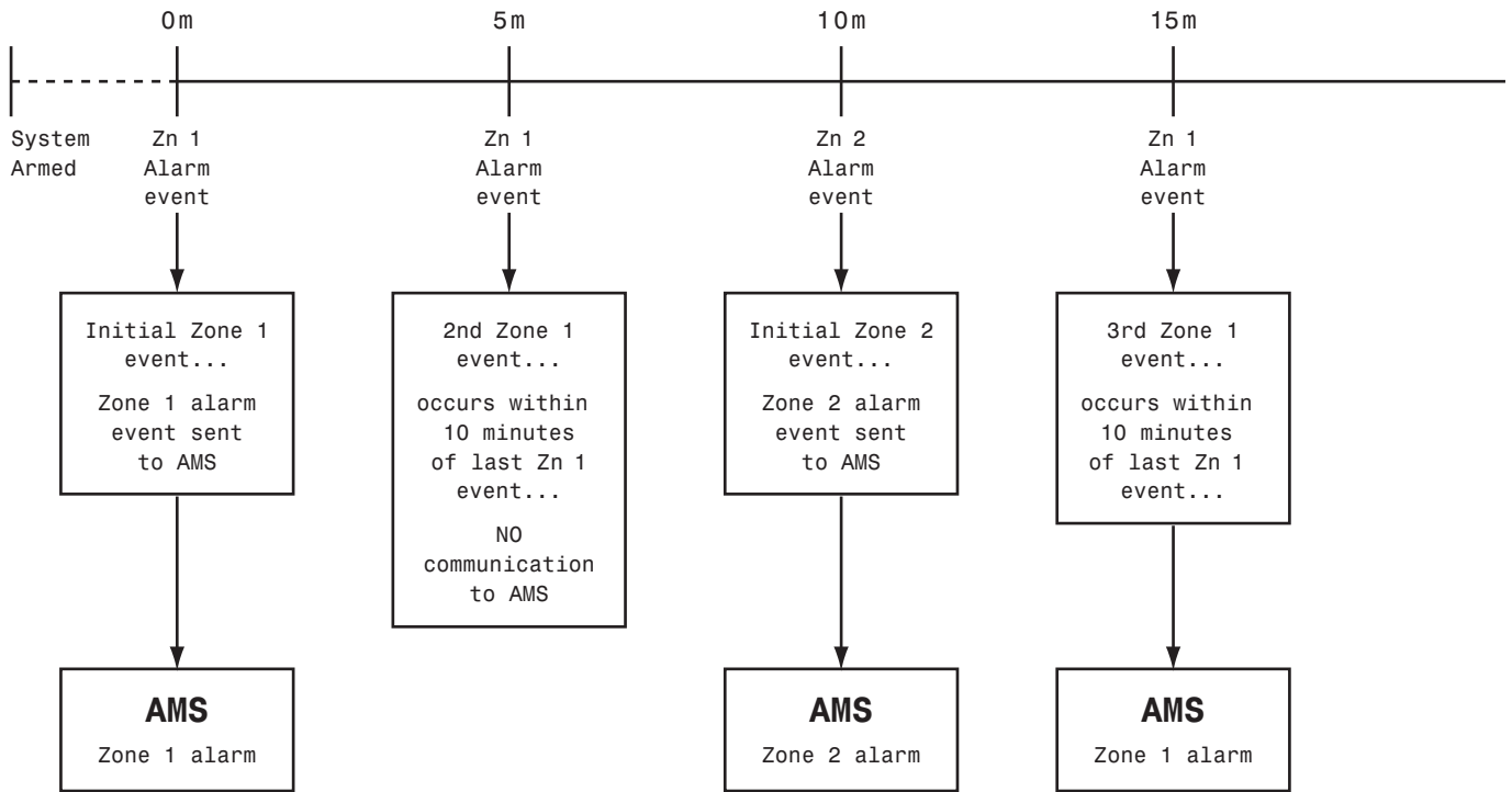
Remote Manager Diagram
